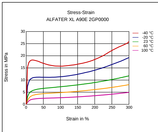
Stress-Strain
